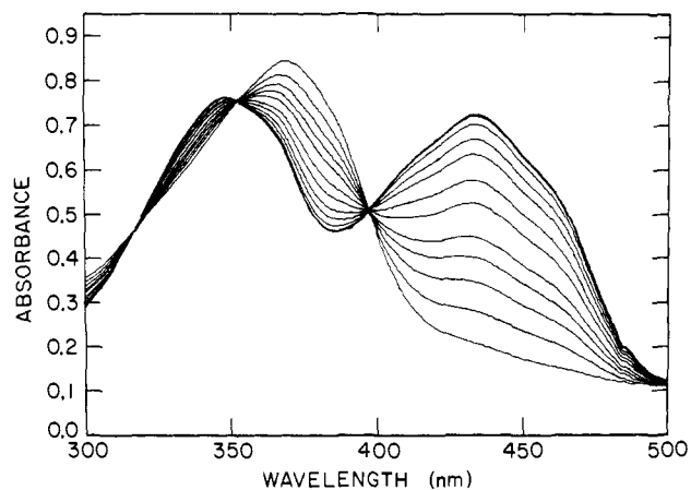
Figure 3. Repetitive scan of the formation of I from VII, pH 11.1, \mu = 1.0 with KCl.
