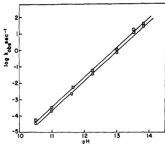
Figure 1. Log k_{\text{obsd}} vs. pH for the specific base catalyzed hydrolysis of I \square III and \circ at 30^\circ , \mu = 1.0 with KCl.
