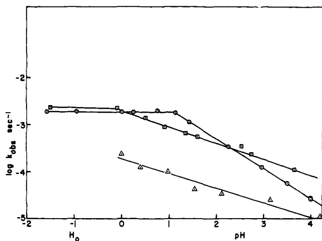
Figure 2. Log k_{\text{obsd}} vs. H_0 or pH for the anaerobic formation of I from VII at 30^\circ , \mu = 1.0 with KCl, \circ ; and \mu = 1.0 with \text{LiClO}_4 , \square . Log k_{\text{obsd}} vs. pH for the cyclization of o -ureidobenzoic acid, \mu = 1.0 with KCl is shown by \triangle .
