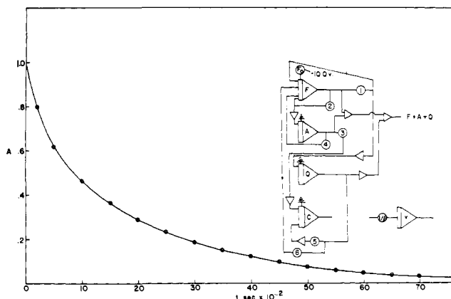
Figure 5. Absorbance vs. time plot for the hydrolysis of IV ( 30^\circ , \mu = 1.0 with KCl, pH 11.2). The points are experimental, and the line was fit by use of an analog computer, the wiring diagram of which is inset.
