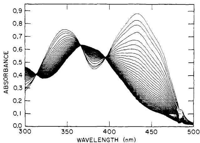
Figure 4. Repetitive scan of the hydrolysis of I, pH 11.2, \mu = 1.0 with KCl.
